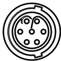
LEMO Socket
