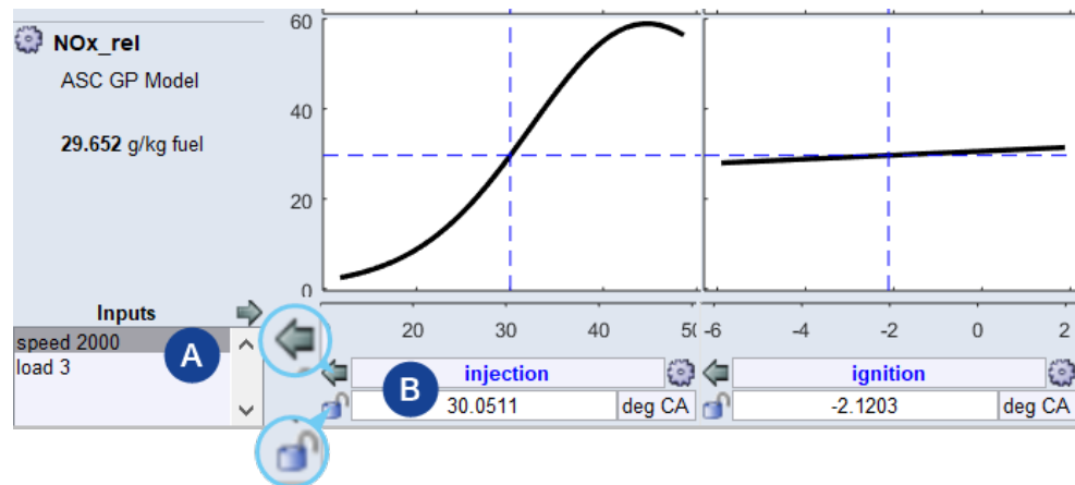
Fig. 5-2: ISP view: Inputs
