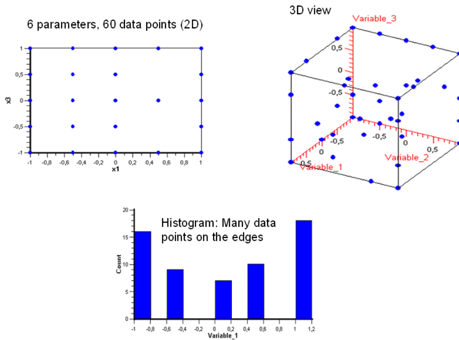
Fig. 4-3: Example for a D-optimal plan
