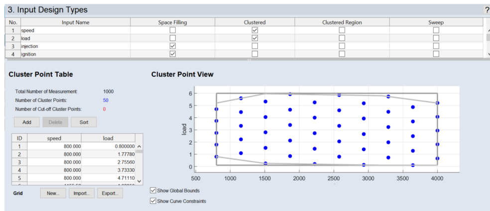
Fig. 7-4: ASCMO-STATIC ExpeDes Step 3: Input Design Types (type Clustered )
