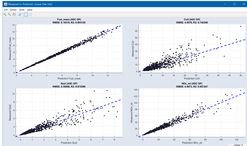
Fig. 4-10: Measuring data and model data
