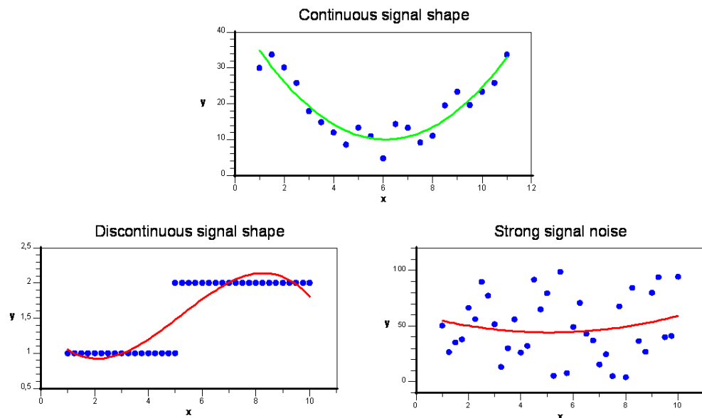
Fig. 4-6: Suitable and unsuitable signal shapes
