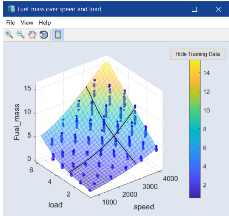
Fig. 6-7: 3D plot of Fuel_mass over speed and load, with training data (blue dots) and color bar
