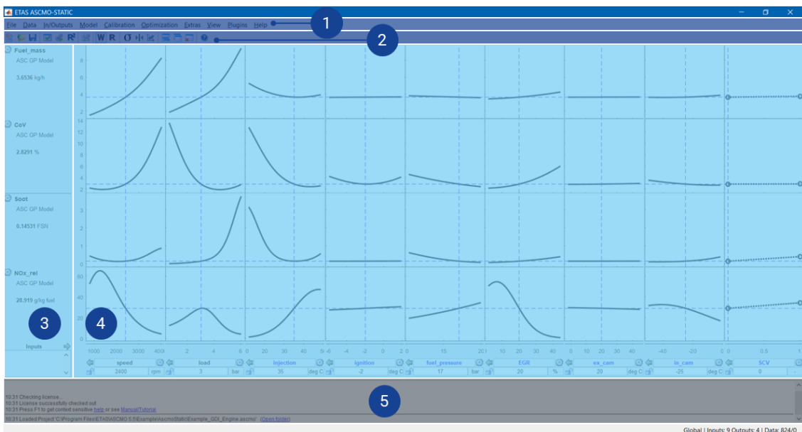
Fig. 5-1: Graphical user interface (GUI) of ASCMO-STATIC (with opened project)
