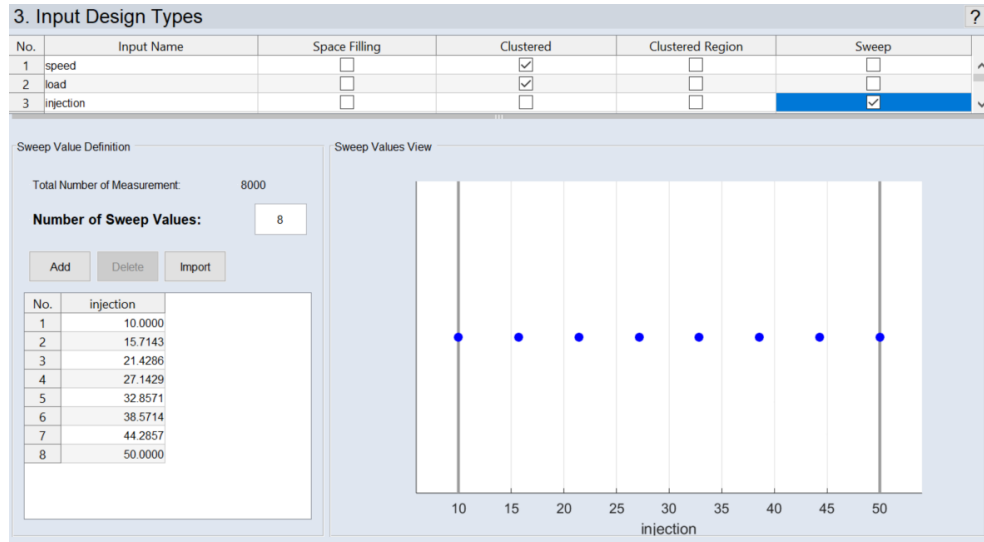
Fig. 7-5: ASCMO-STATIC ExpeDes Step 3: Input Design Types (type Sweep )
