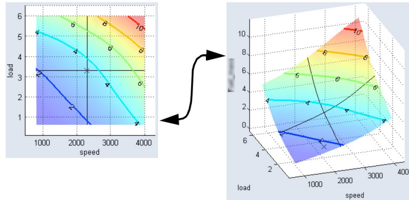
Fig. 6-8: 3D plot of Fuel mass over speed and load, with contour lines
