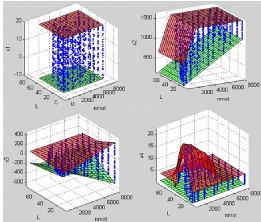
Fig. 4-5: Measuring points and experiment space limits
