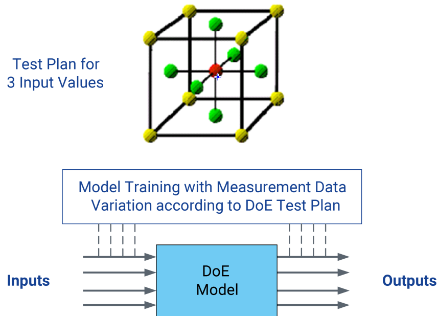
Fig. 4-1: Model training with data from the DoE plan
