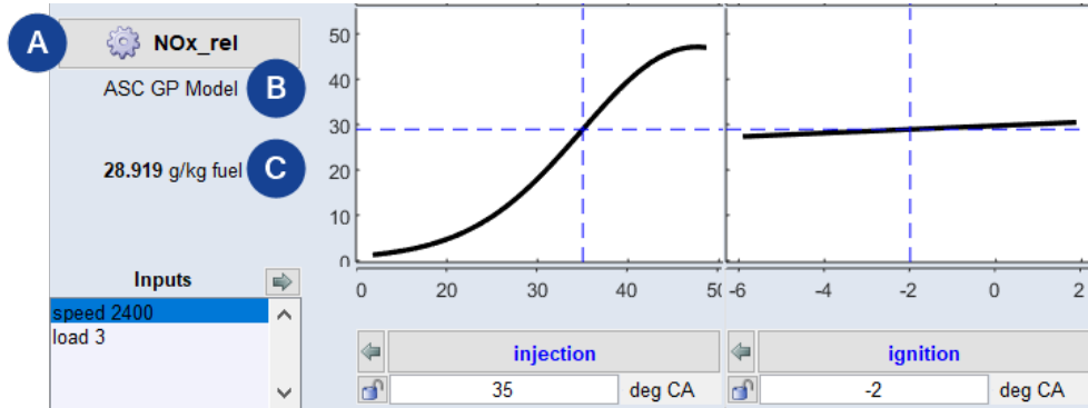
Fig. 5-3: ISP view: Outputs
