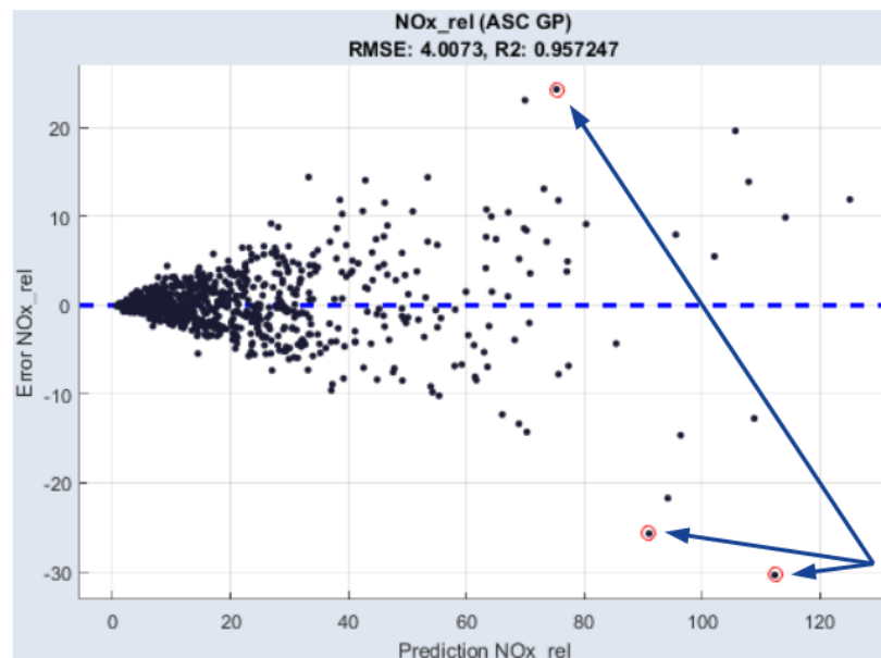
Fig. 6-4: Absolute error versus model prediction
