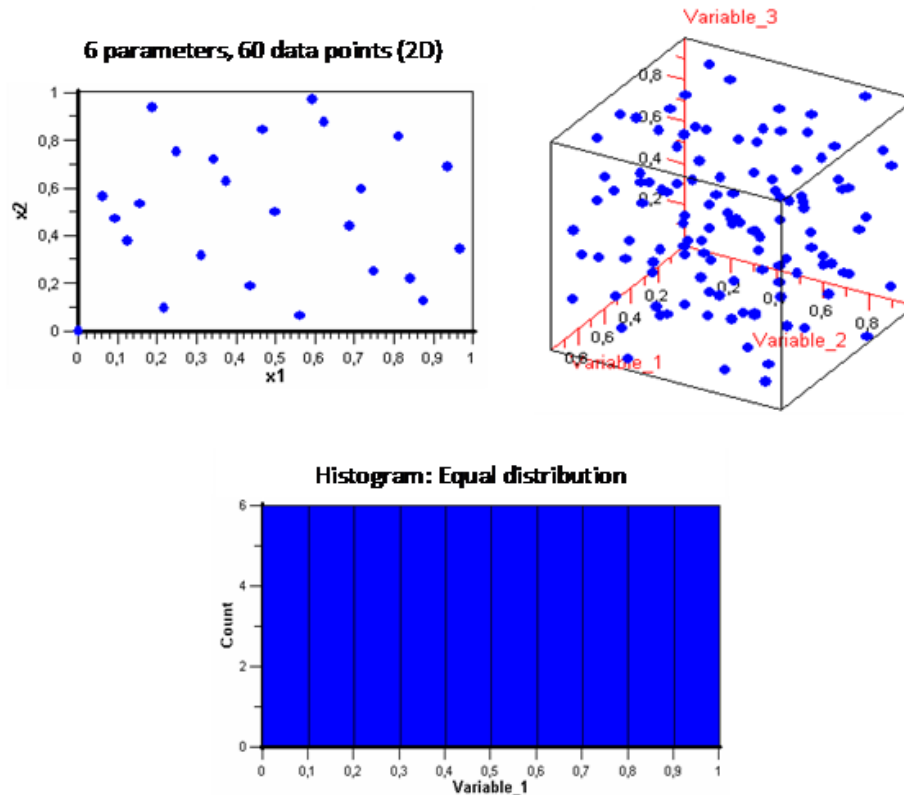
Fig. 4-4: Example for a space-filling experiment plan
