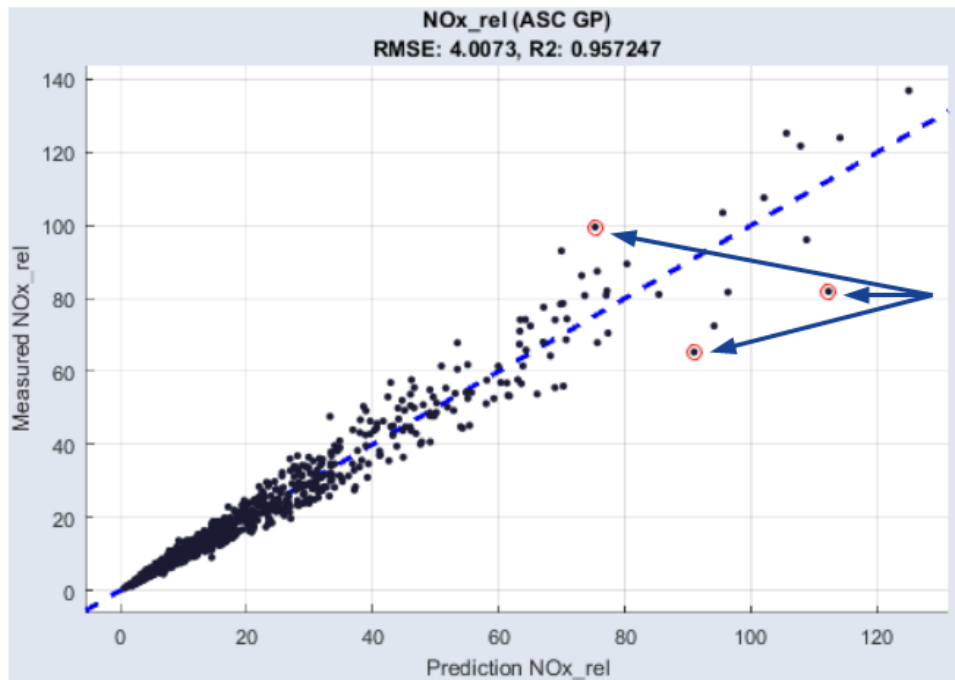
Fig. 6-2: Outliers in the Measured vs. Predicted display
