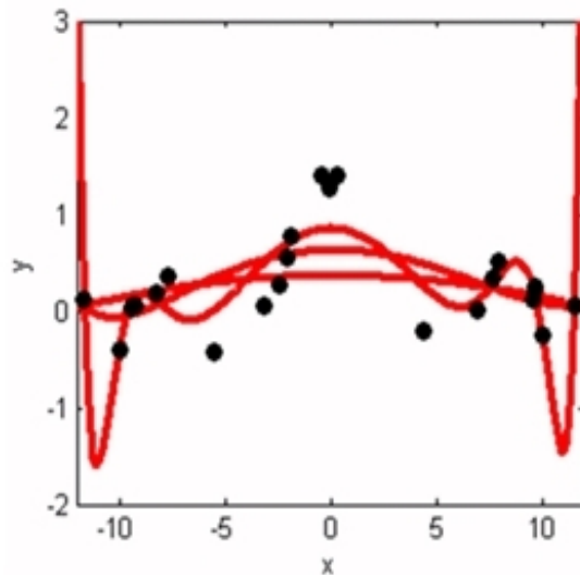
Fig. 4-8: Fit to measuring data using polynomials
