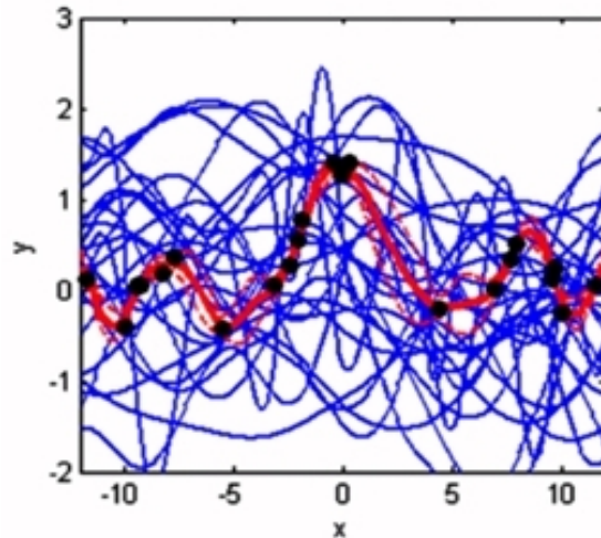
Fig. 4-9: Fit to measuring data in ASCMO-STATIC
