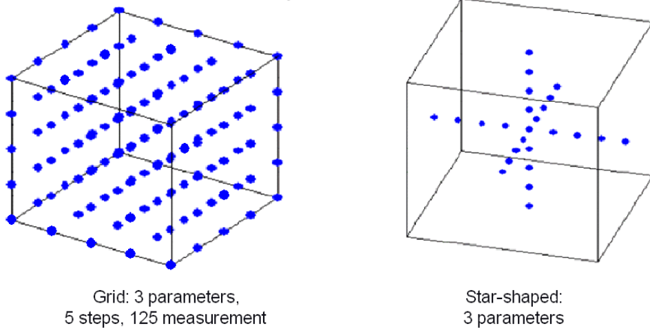
Fig. 4-2: Grid measurement and star-shaped measurement of the experimental space
