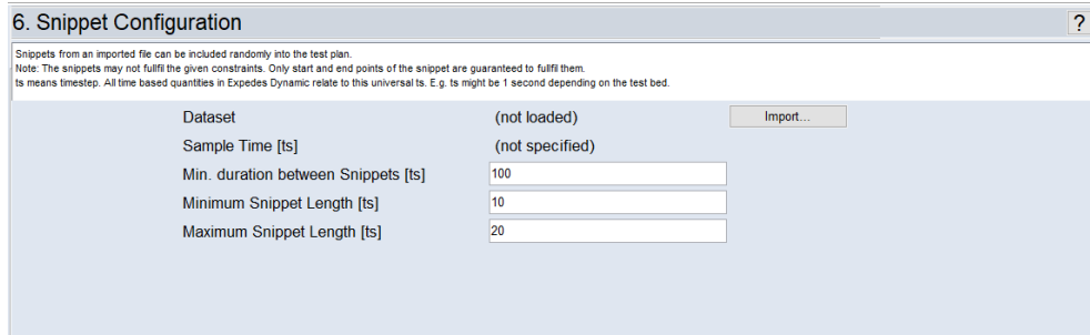
Fig. 6-7: ASCMO-DYNAMIC ExpeDes Step 6: Snippet Configuration
