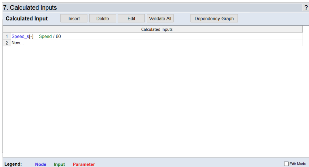
Fig. 6-8: ASCMO-DYNAMIC ExpeDes Step 7: Calculated Inputs
